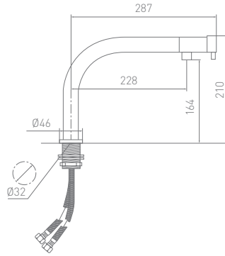
MB238 High Spout Mono Basin Mixer
