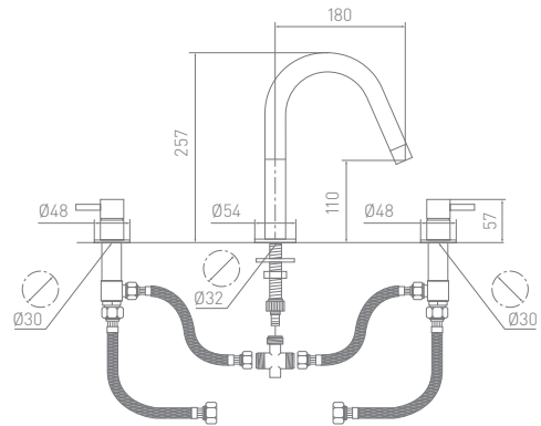
MB278 Wall Mounted Basin Mixer
