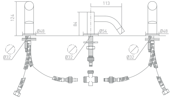
CB203 3-piece Low Spout Basin Mixer
