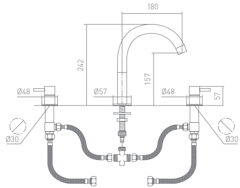
MB253 3-piece High Spout Basin Mixer
