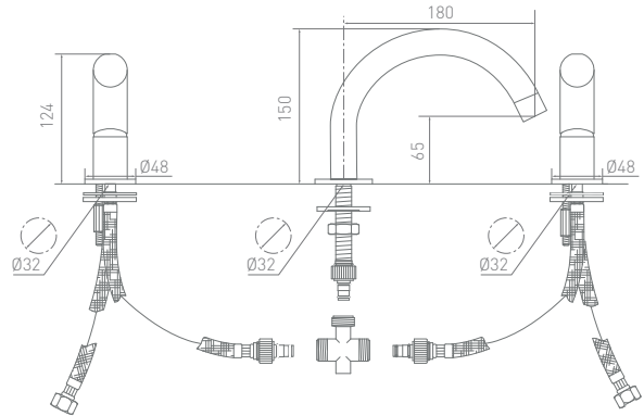
CB201 3-piece Basin Mixer
